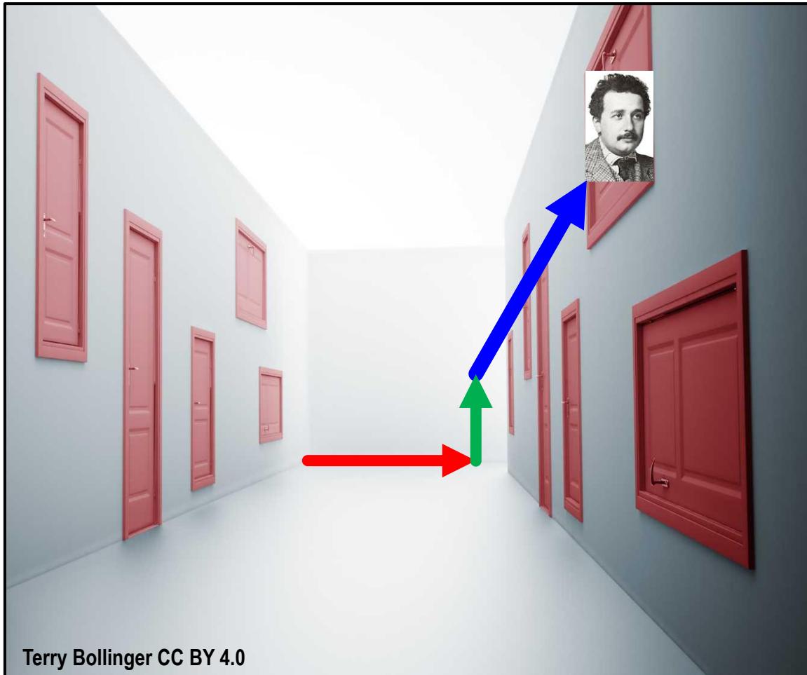
Fig 1. Einstein's observation that rigidity underlies all point-location systems
