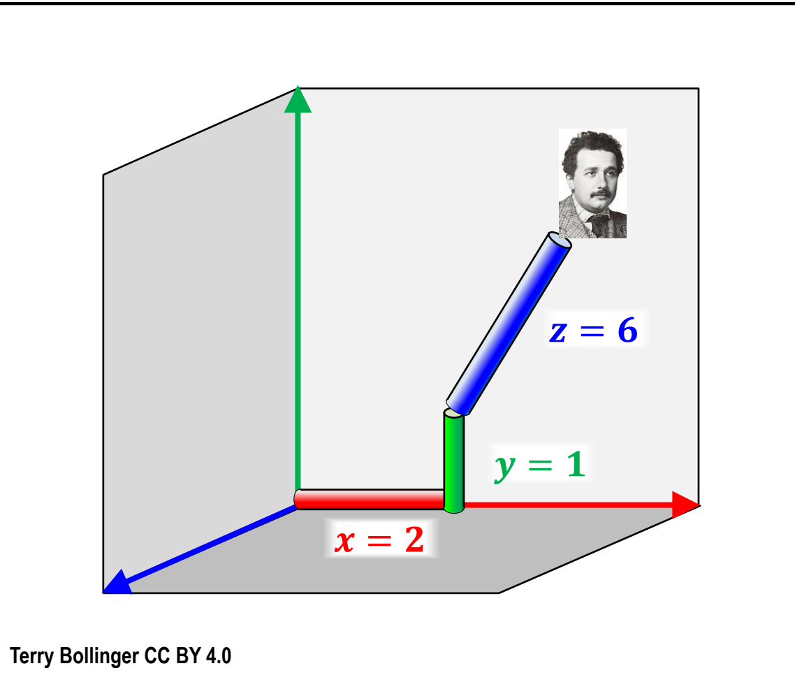
Fig 1. Einstein's observation that rigidity underlies all point-location systems
